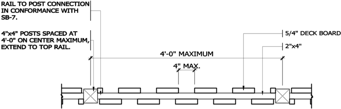
TOP VIEW 1" = 1'-0"
