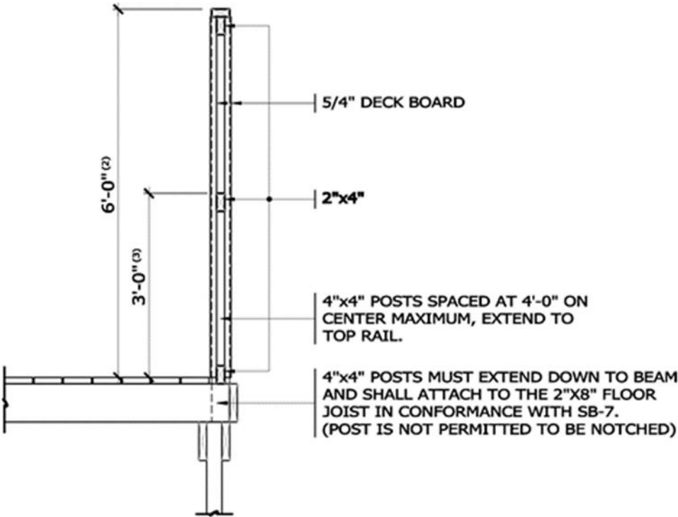
SECTION 1/2" = 1'-0"
